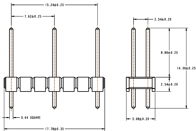
Figure B3.1-1 Connector Diagram
